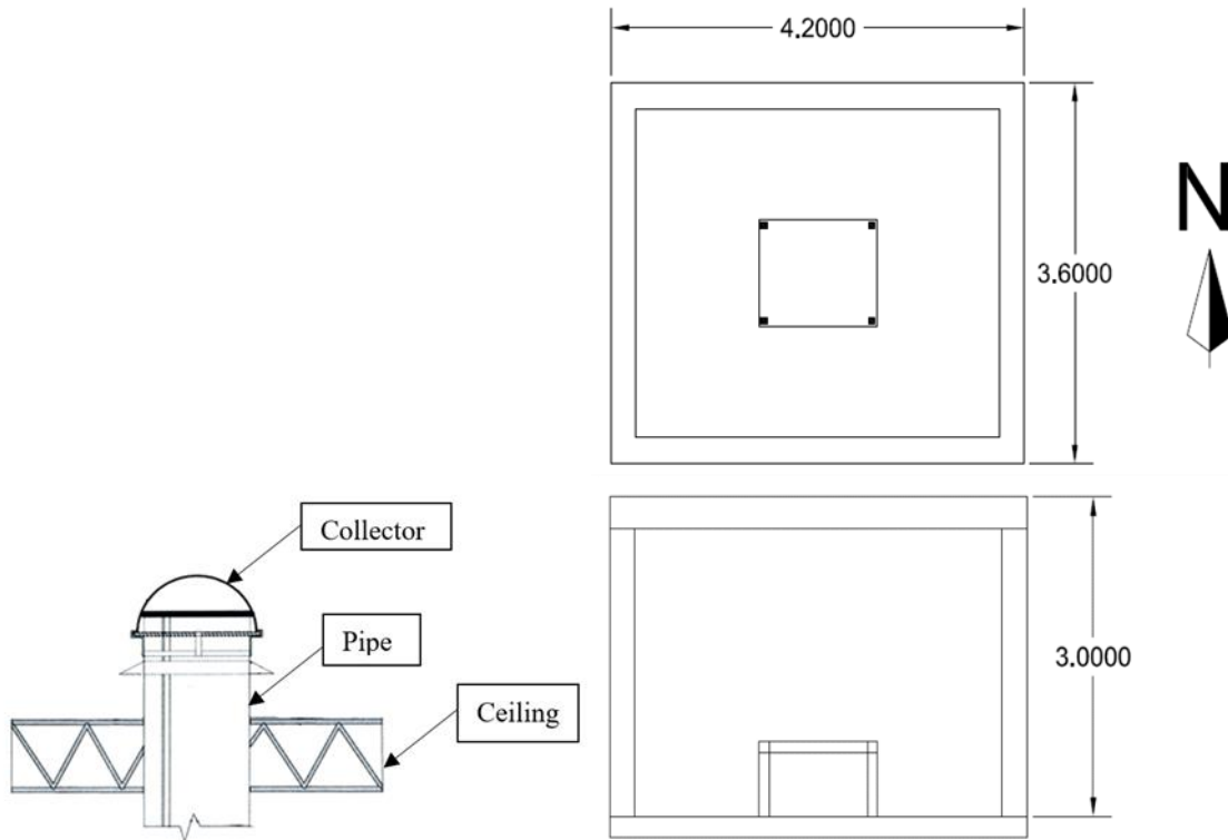
Fig. 4: light tube section
