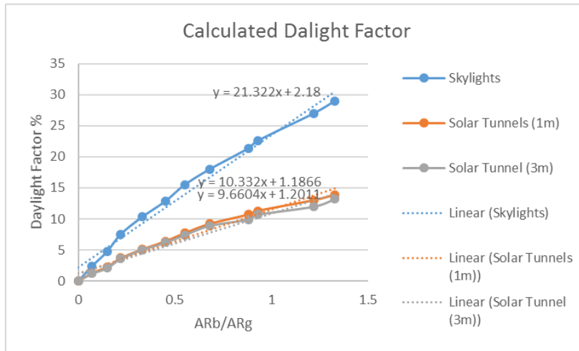
Fig. 7: Calculated Daylight factor for three typologies of systems of a number of devices
